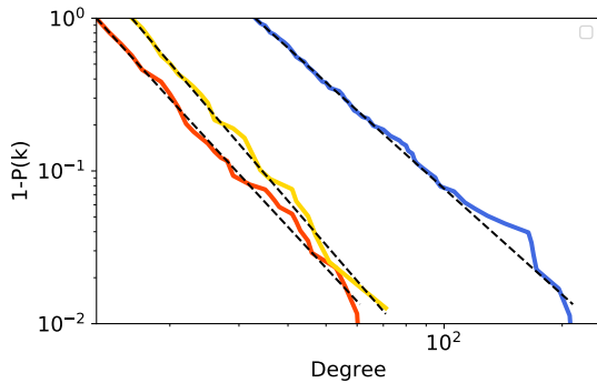
Fig. 1. Complementary Cumulative Probability 1-P(k) plotted as a function of degree k (solid lines) of the labour flow network on log-log scales, with fitted power law (dashed lines). The blue line shows the degree distribution of a single-layer network, where power-law fitting [11] finds b = 3.30 . The red and yellow lines show the degree distributions of high-skilled and low-skilled layer of the two-layer multiplex network, power-law fitting finds b = 3.74 and b = 3.94 respectively.
